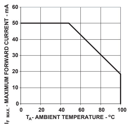
Figure 3. Forward current vs. ambient temperature.
